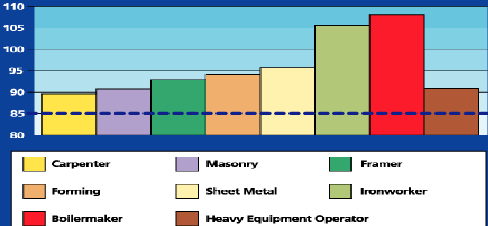
Graph 1: Average dB(A) For Some Construction Trades / Activities
